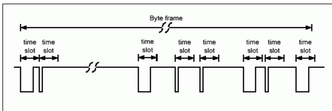
Figure 9. Bit-to-Bit timing flexibility.
