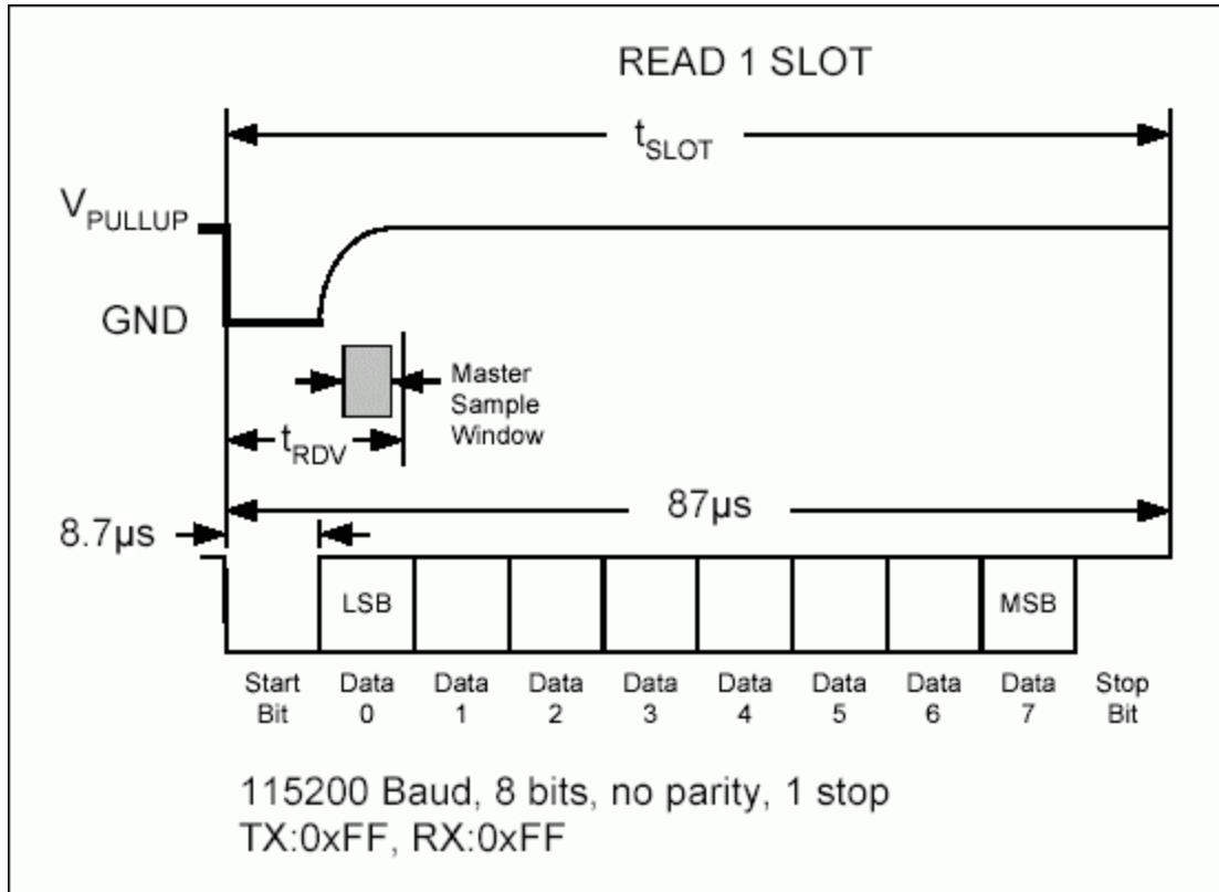
Figure 6. Read 1 time slot.
